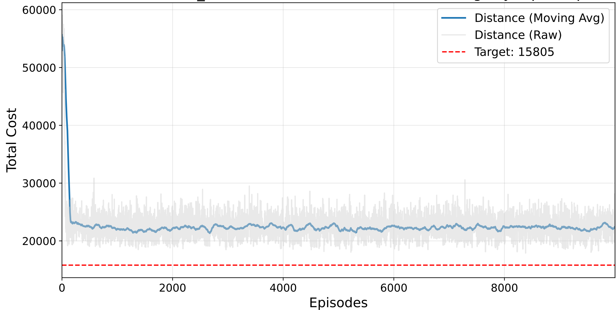
Final RANDOM_SEARCH Masked AutoRL-SOP Training - ry48p.1.sop
